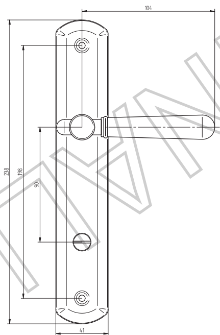
DASA NOVA WC OUT 90mm PRAVA-MS-BR
