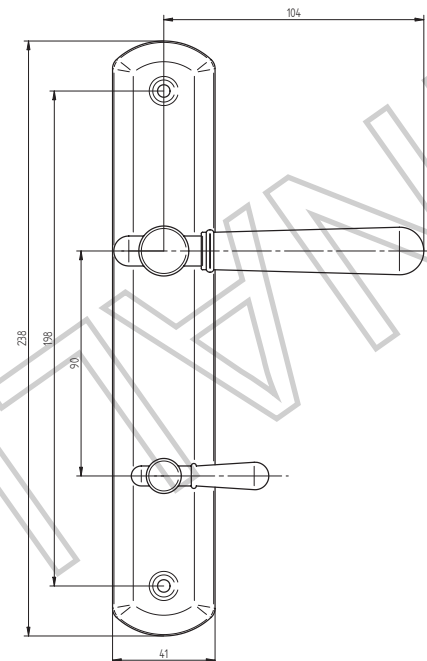
DASA NOVA WC IN 90mm PRAVA-MS-BR
